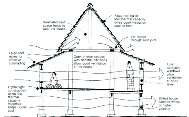
Gambar 13. Climatic Design of the Malay House (Sumber : Yuan, 1987)
